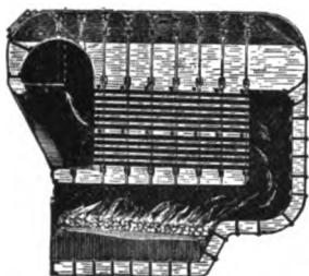
FIG. 30.—MARINE TUBULAR BOILER.
